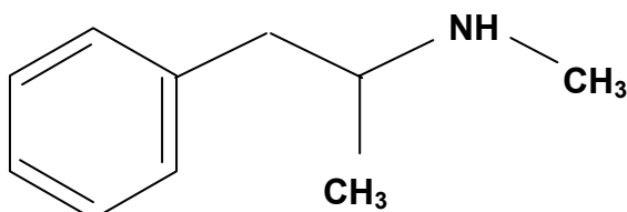
Figure 1: Amphetamine and methamphetamine molecules
