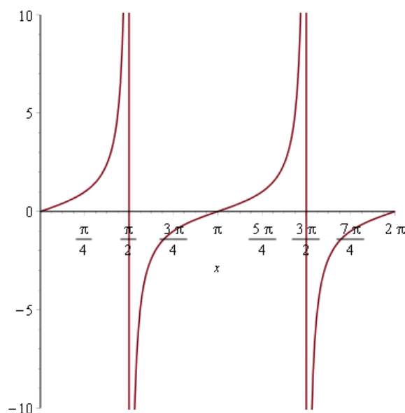
Figure 2.1: Plot of \tan x
