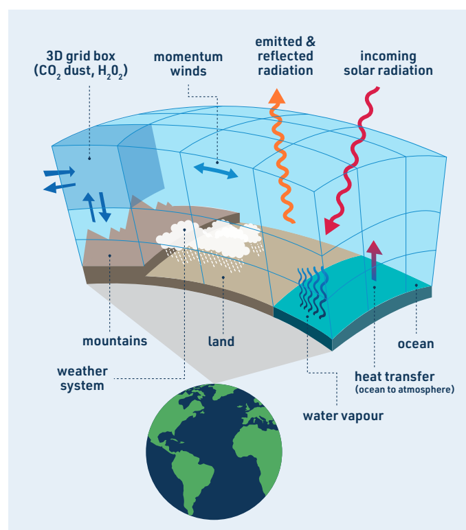
Figure 1: Illustration of the three-dimensional grid of a climate model. This is a simplification, many more processes are included in the atmosphere, ocean and land. Image: Adapted from Earth's Climate: Past and Future by William F. Ruddiman.
