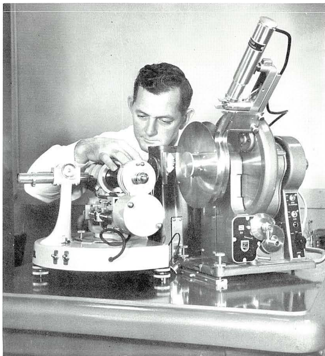
x-ray diffractometer
