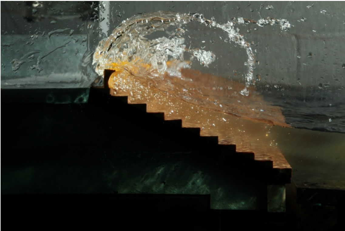
Figure 2: Stepped concrete seawall - Configuration B (6 m AHD Crest, with wave return wall) during 10 year ARI event, present day
