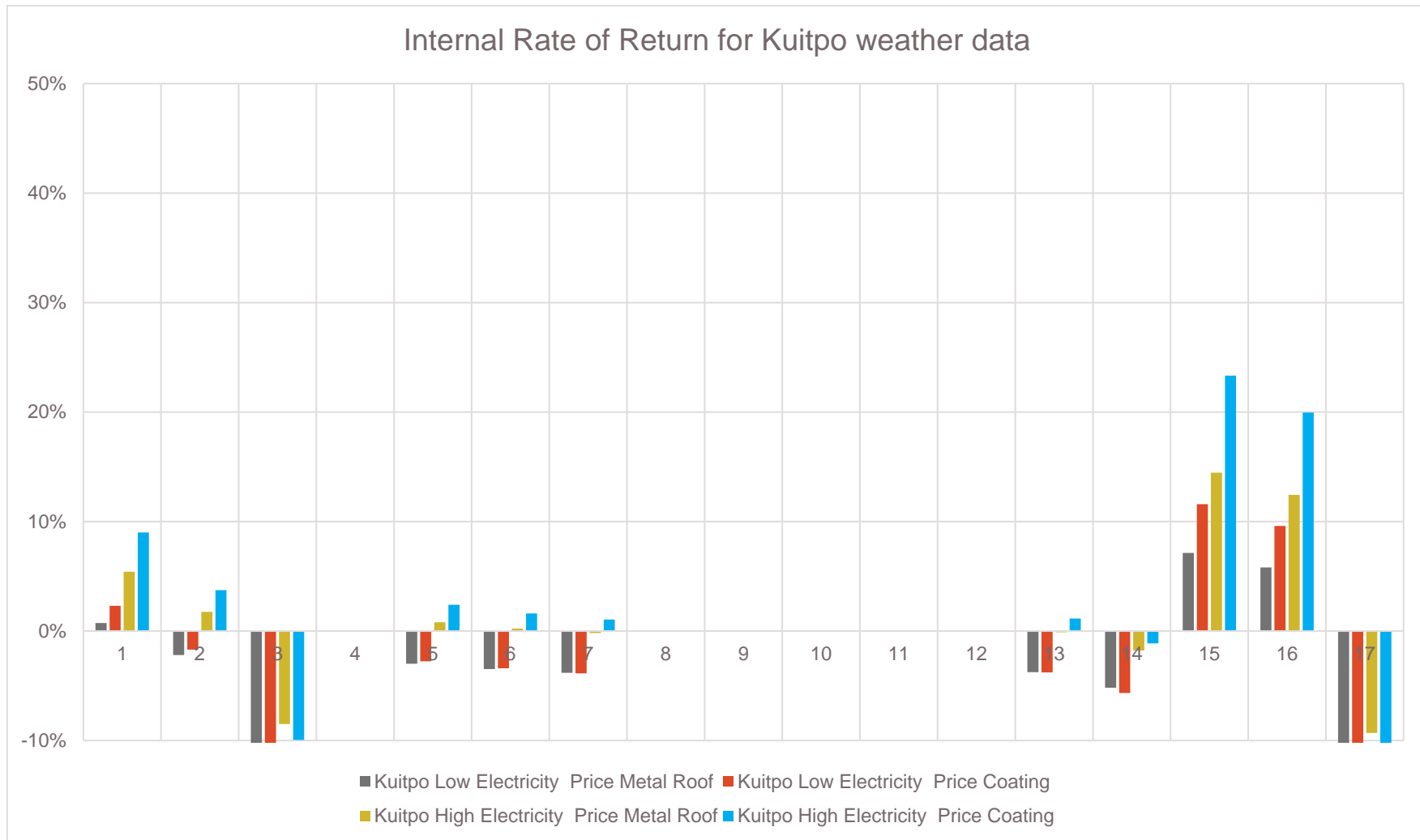
Figure 64 Internal Rate of Return for the buildings for Kuitpo weather conditions
