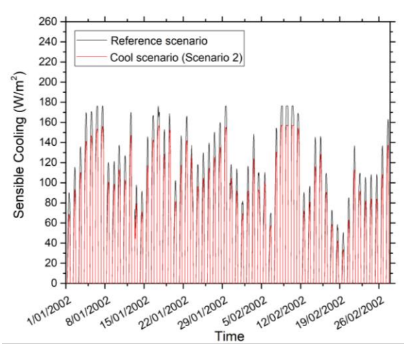
Figure 59 Sensible cooling load in cool roof with modified urban temperature scenario (scenario 2) and reference scenario for a typical low-rise shopping mall centre-existing building in Roseworthy station
