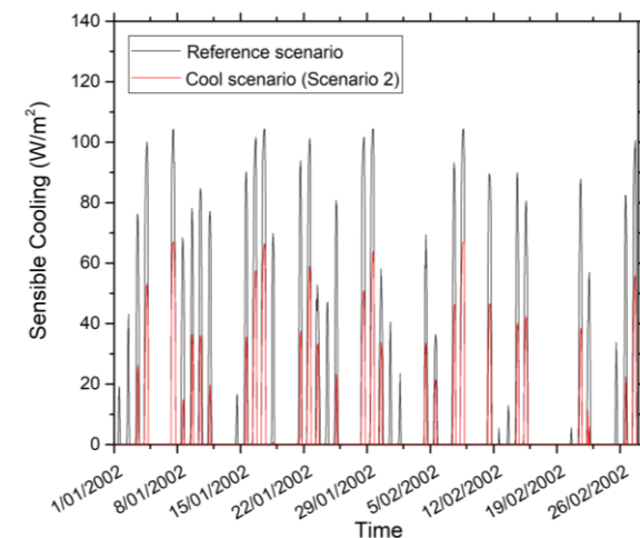
Figure 28 Sensible cooling load in cool roof with modified urban temperature scenario (scenario 2) and reference scenario for a low-rise office building without roof insulation-existing building in Kuitpo station
