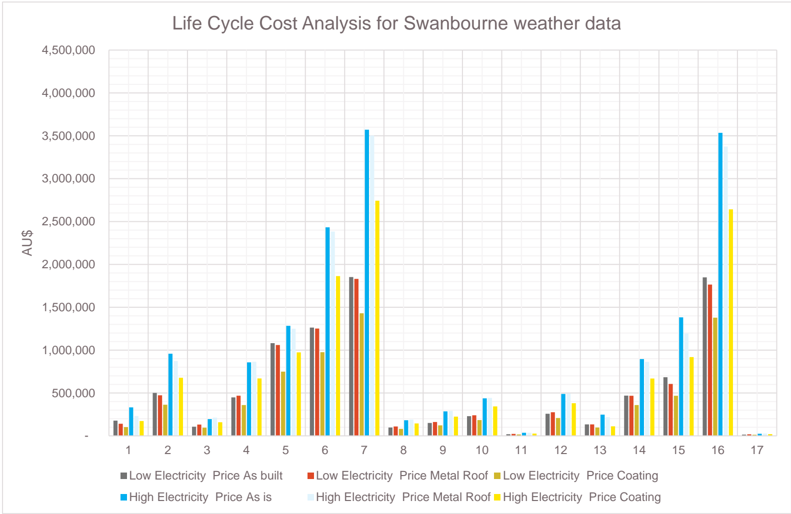
Figure 30 Life Cycle Cost for the buildings for Swanbourne weather conditions
